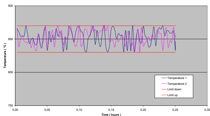
Difference between temperature - BS EN 50200
