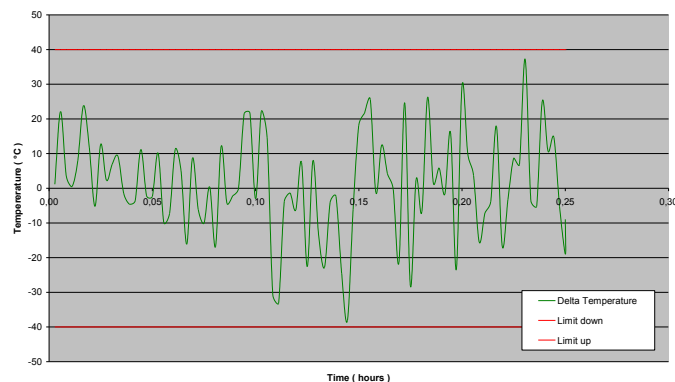
Difference between temperature - BS EN 50200
